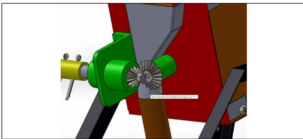
Fig.3 Assembly design of bevel and pinion gear
