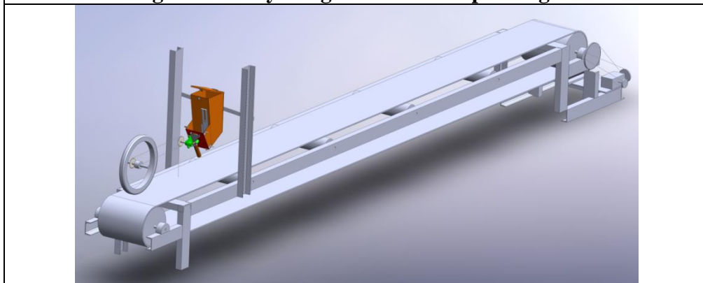
Fig.4 Whole assembly of experimental lab-setup in solid works
